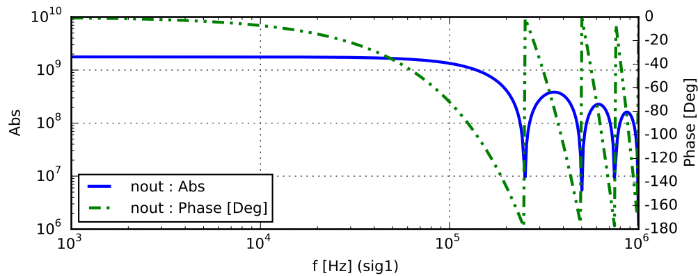
Figure 5.11: FINESSE example: Michelson sideband output from a gravitational wave
