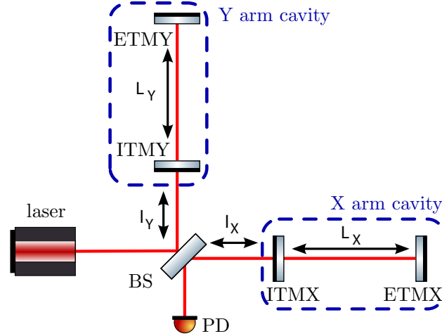
Figure 7.3: Optical layout of a Michelson interferometer with arm cavities.
