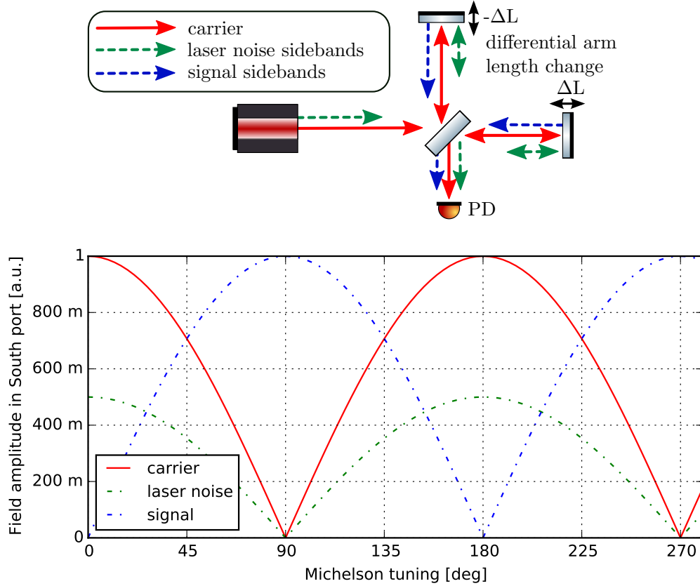
Figure 5.7: A Michelson interferometer shown with three types of light field: the ‘carrier’, representing the undistorted laser input field, ‘laser phase noise sidebands’, which enter the interferometer with the carrier, and ‘signal sidebands’, which are phase modulation sidebands caused by differential arm length motion. All three fields leave the interferometer through both output ports (here only the detector in the South port is shown). The graph shows the amplitude of the three light fields in the South port as a function of the Michelson tuning (differential arm length change). At 0 degrees the Michelson is on a bright fringe and at 90 degrees on a dark fringe .
