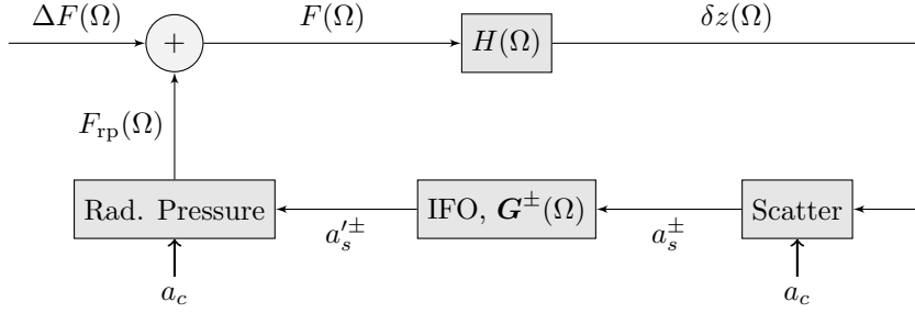
Figure 6.8: A generic view of a closed-loop opto-mechanical transfer function for a suspended mirror with mechanical susceptibility H(\Omega) . Due to some motion \delta z(\Omega) of a mirror the light is scattered from the carrier. The IFO plant describes the optical transfer function of the sidebands propagating through the interferometer and back to the mirror in question. The interference of these then creates some radiation pressure force which is fed back into the mirror. Here a_c is the carrier field at the mirror in question.
