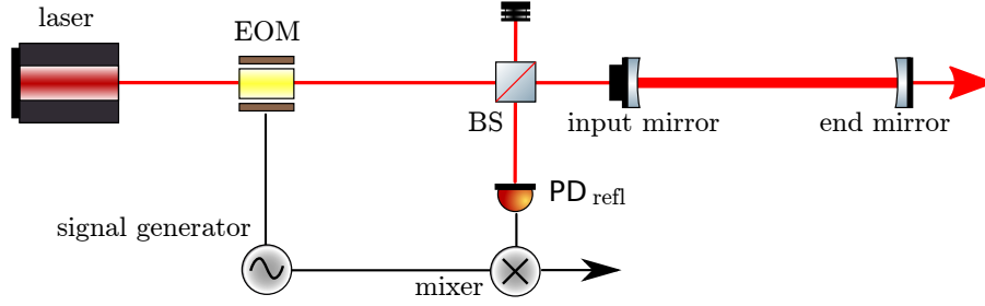
Figure 8.7: Typical setup for using the Pound–Drever–Hall scheme for length sensing and with a two-mirror cavity: the laser beam is phase modulated with an electro-optical modulator (EOM). The modulation frequency is often in the radio frequency range. The photodiode signal in reflection is then electrically demodulated at the same frequency.
